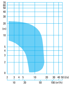
CH... -2 pole
